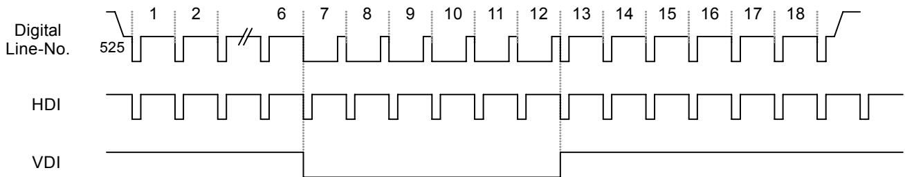
Fig. 87 525p Relation between HSYNC and VSYNC
