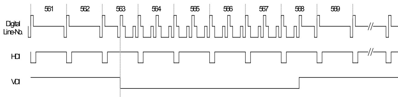
Fig. 103 1125i (1080i) Relation between HSYNC and VSYNC(2)
