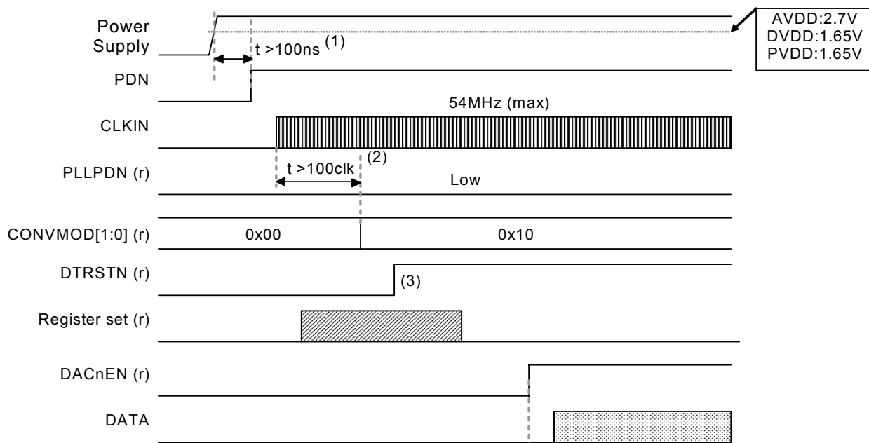
Fig. 14 Power-Up sequence (To set High Speed Video DAC mode after power-up)
