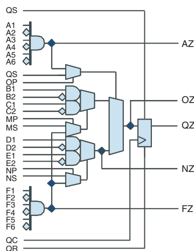
Figure 3: QuickRAM Logic Cell
