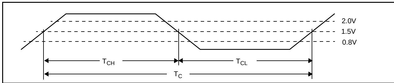
Figure 7. Timing Waveform
