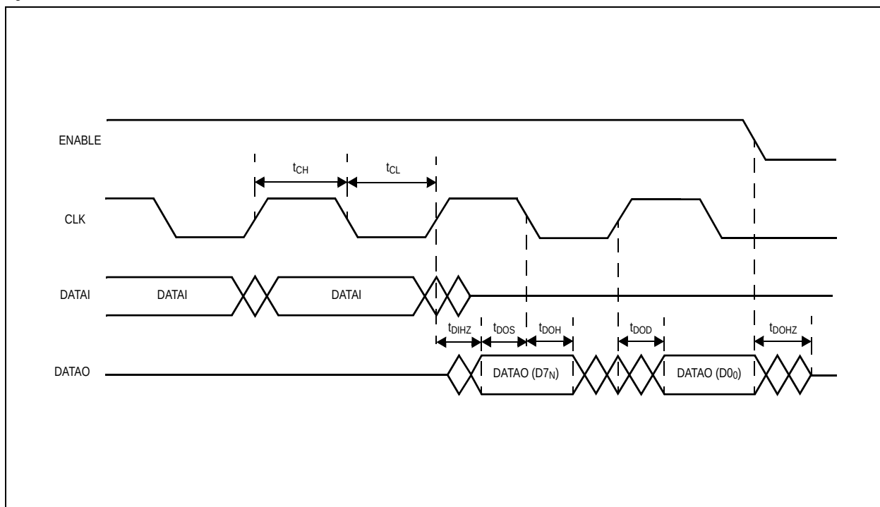
Figure 4. Read Data
