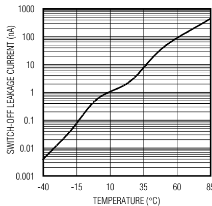
SWITCH-OFF LEAKAGE CURRENT vs. TEMPERATURE
