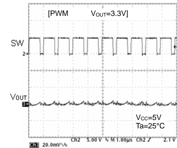
Figure 16. SW Waveform ( I_o=3A )
