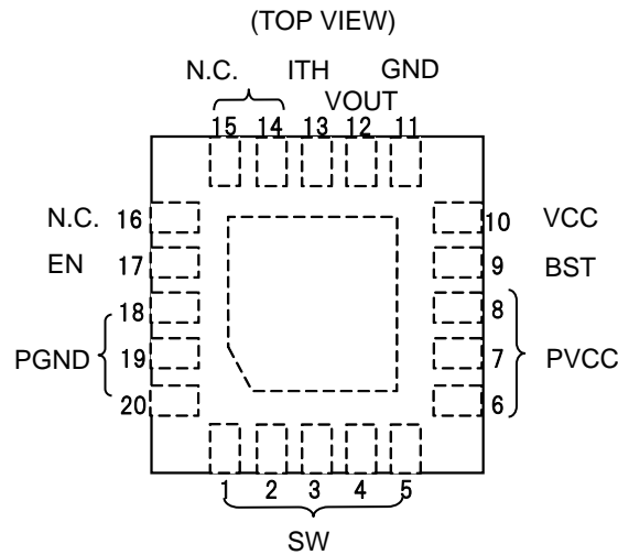
Figure 2. Pin Configuration
