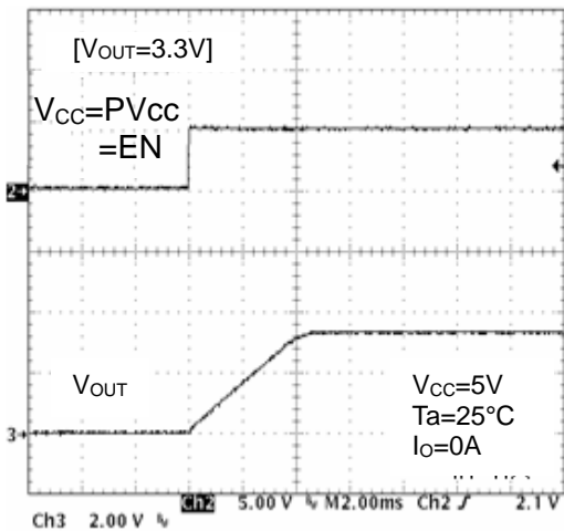
Figure 14. Soft-Start Waveform
