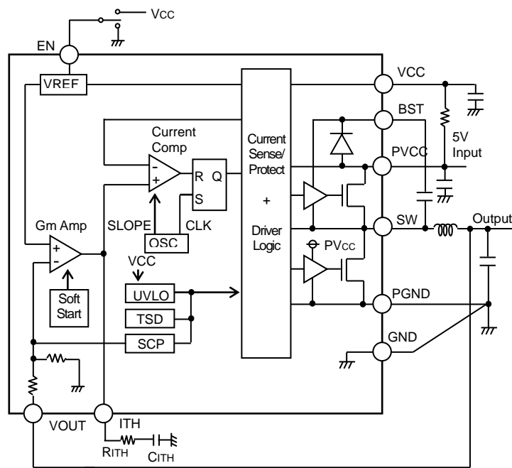
Figure 3. Block Diagram
