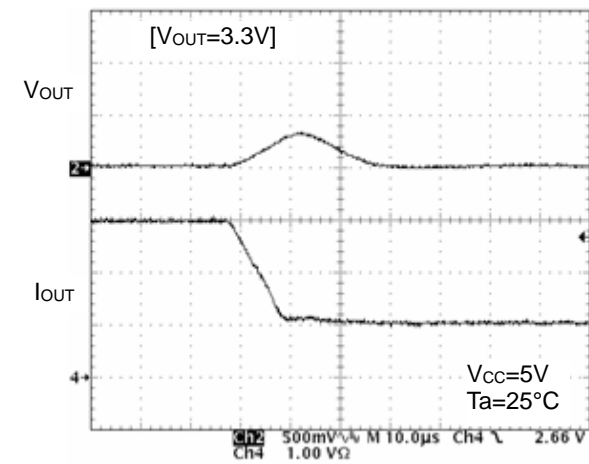
Figure 18. Transient Response ( I_o=3A to 1A , 10\mu s )
