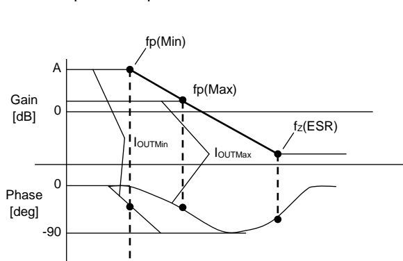
Figure 31. Open Loop Gain Characteristics
