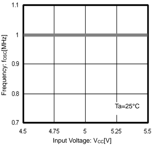
Figure 13. Frequency vs Input Voltage
