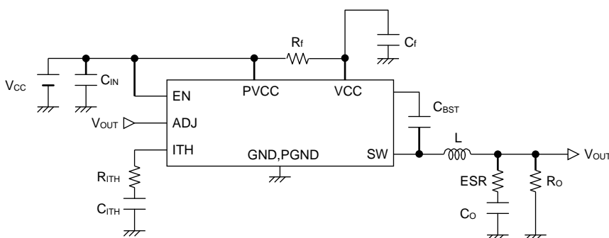
Figure 33. Typical Application
