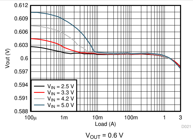
Figure 8-4. Load Regulation
