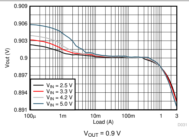
Figure 8-8. Load Regulation
