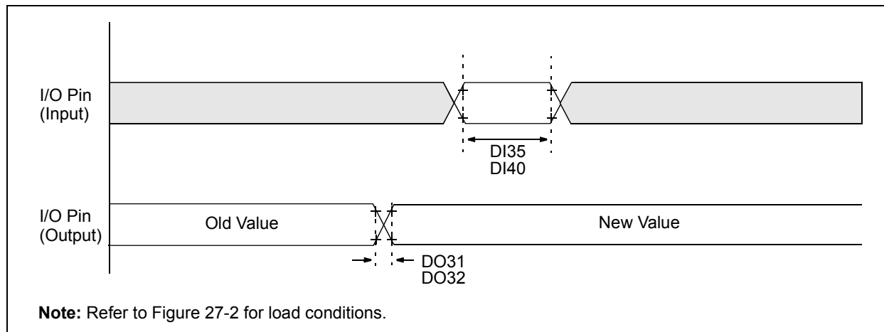
FIGURE 27-4: CLKO AND I/O TIMING CHARACTERISTICS
