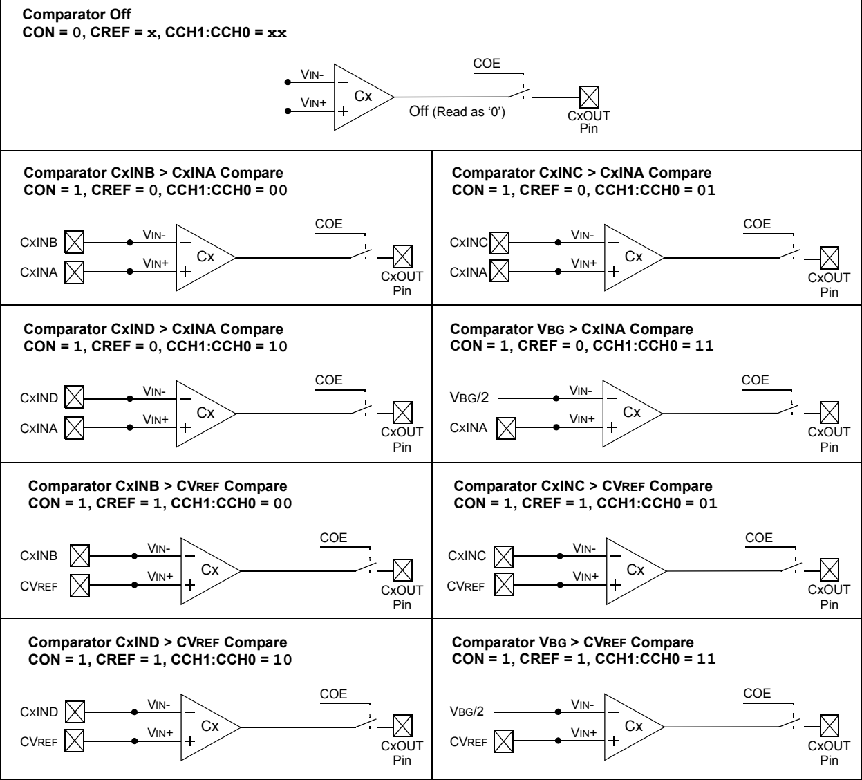
FIGURE 21-2: INDIVIDUAL COMPARATOR CONFIGURATIONS
