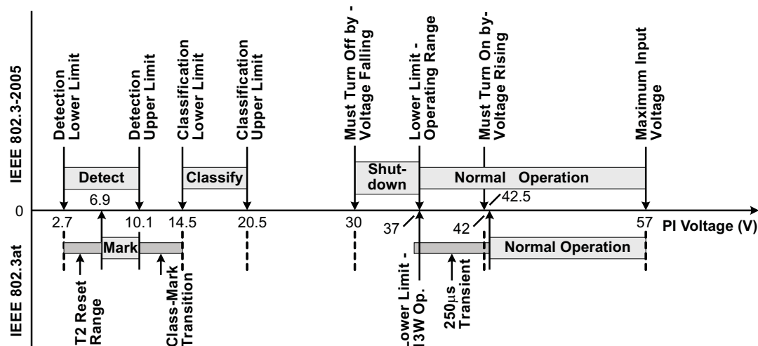
Figure 20. Operational States for PD
