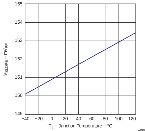
Figure 14. Current Slope Compensation Voltage vs Temperature
