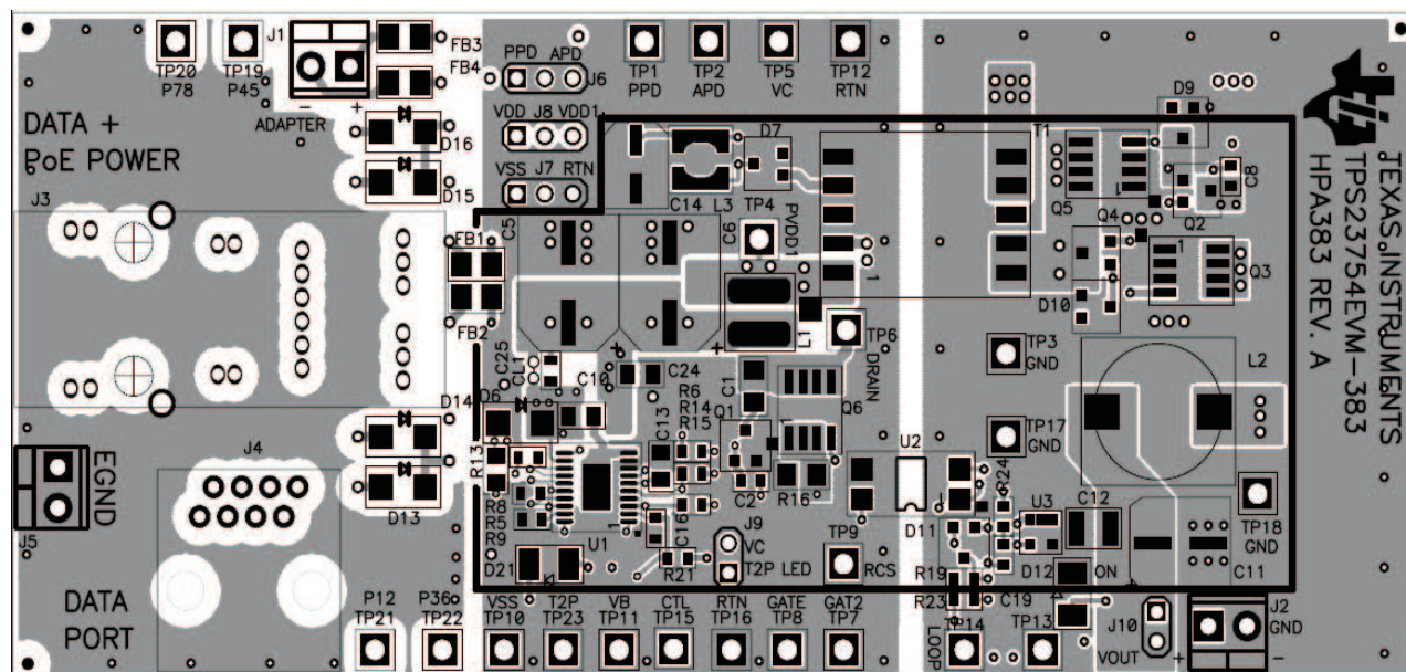
Figure 39. TPS23754EVM-383 EVM Parts Placement and Example Layout
