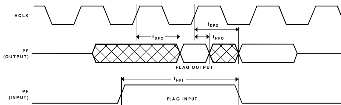
Figure 12. Programmable Flags Cycle Timing
