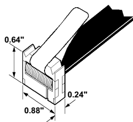
Figure 9. JTAG Pod Connector Dimensions
