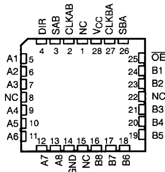
SN54ABT646A ... FK PACKAGE (TOP VIEW)
