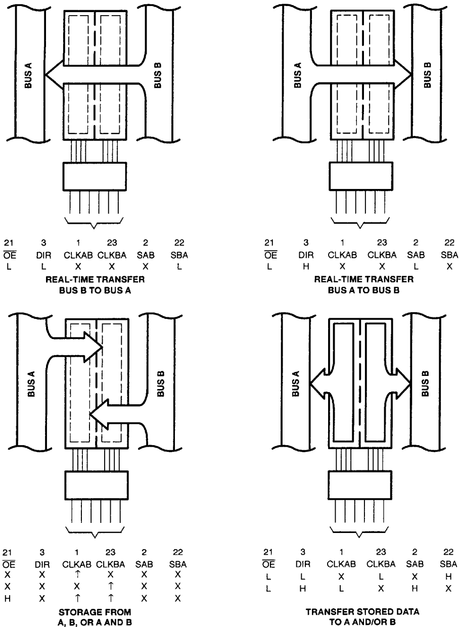
Figure 1. Bus-Management Functions
