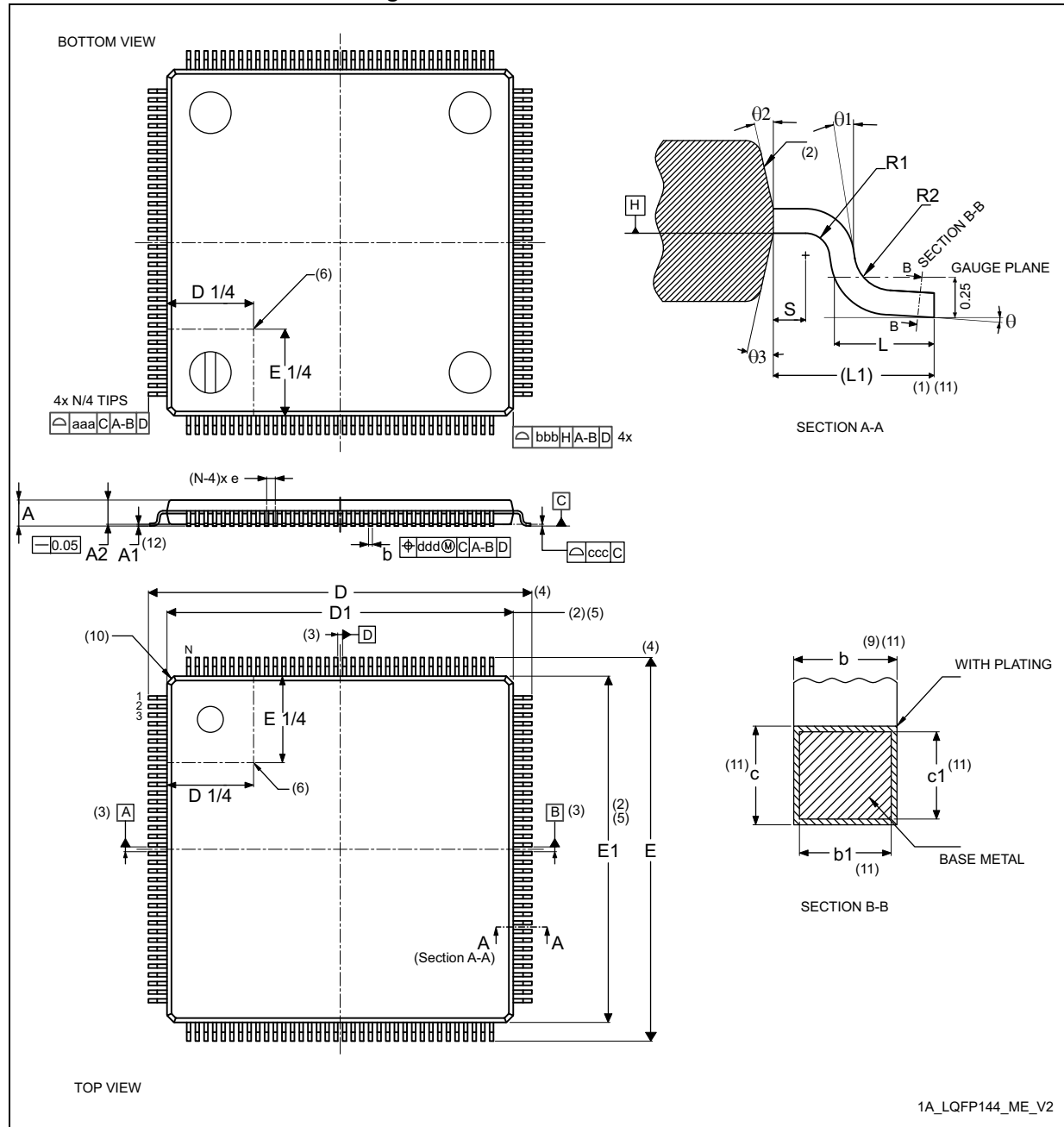
Figure 54. LQFP144 - Outline (15)
