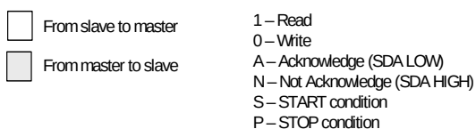
Figure 10. I 2 C Read Operation
