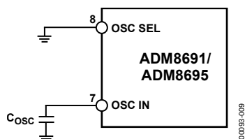
Figure 18. External Capacitor
