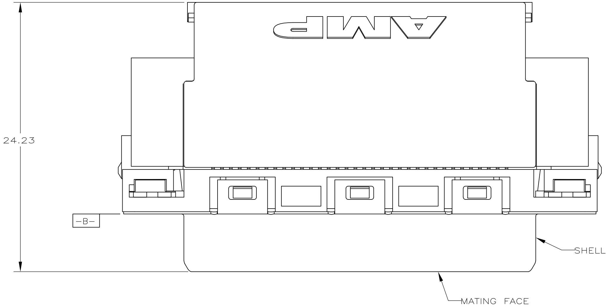
VIEW F—F
