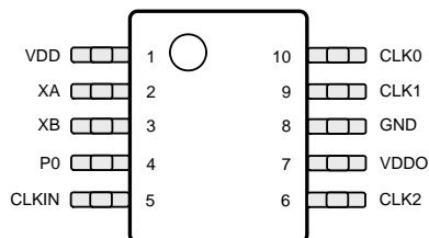
Si5350C 10-MSOP Top View
