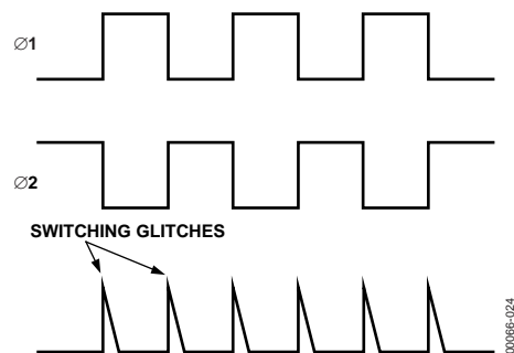
Figure 24. Switching Glitches
