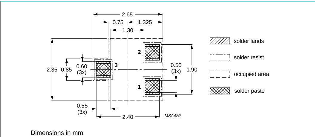
Fig 22. Reflow soldering footprint SOT323 (SC-70)
