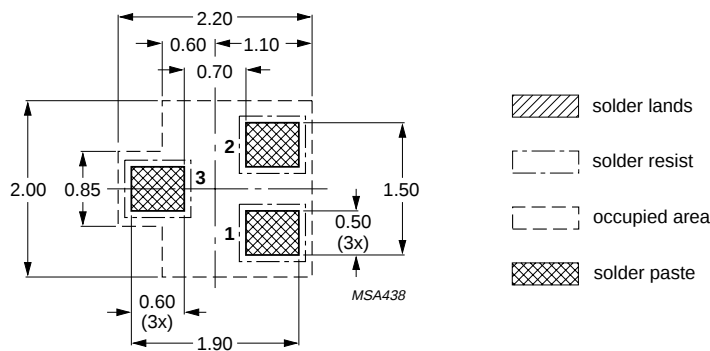
Fig 28. Reflow soldering footprint SOT416
