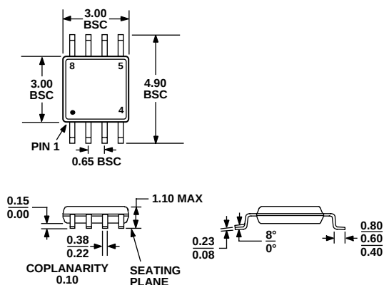
Figure 26. 8-Lead Micro Small Outline Package [MSOP] (RM-8)
