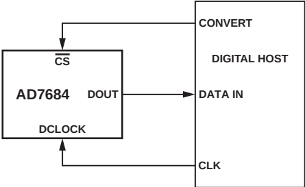
Figure 25. Connection Diagram
