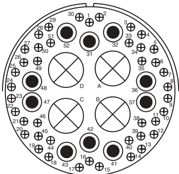
Insert Arrangement 48-51 Service Rating A Number of Contacts 42 Contact Size 16
