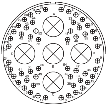
Insert Arrangement 48-52 Service Rating A Number of Contacts 56 Contact Size 16
