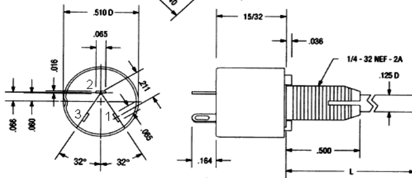
LOCKING BUSHING
