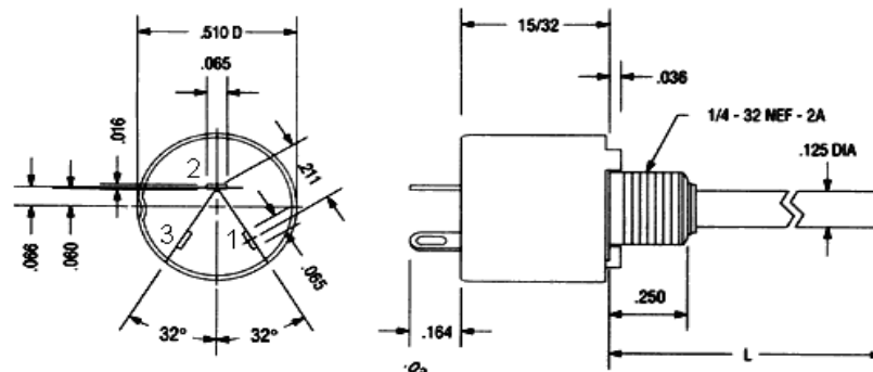
STANDARD BUSHING
