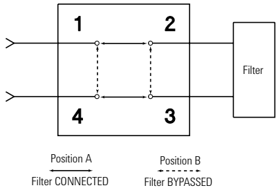
Figure 3. Drop-out switch
