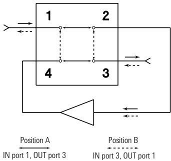
Figure 2. Signal reversal
