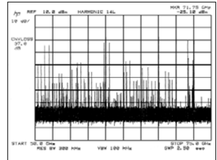
50 to 75 GHz sweep without preselection
