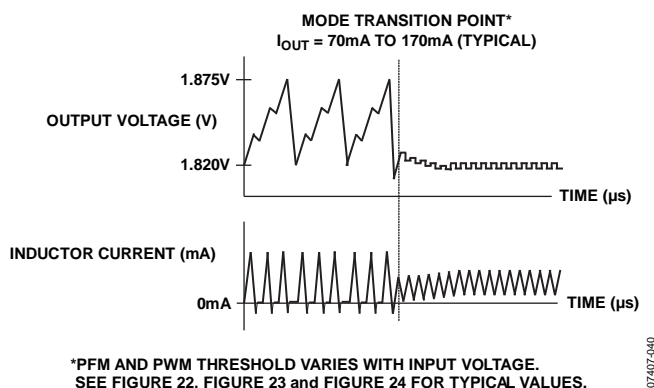
Figure 53. PFM-to-PWM Transition Point, V_{OUT} = 1.82\text{ V}
