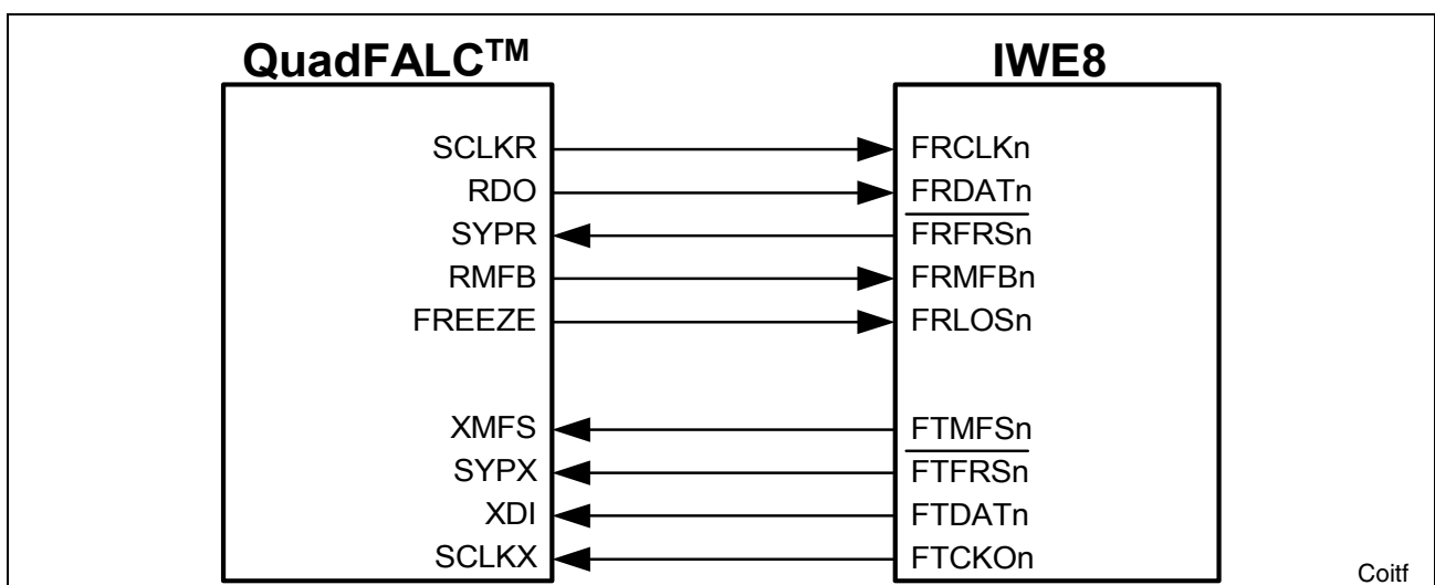
Figure 22 Connection of IWE8 to QuadFALC
