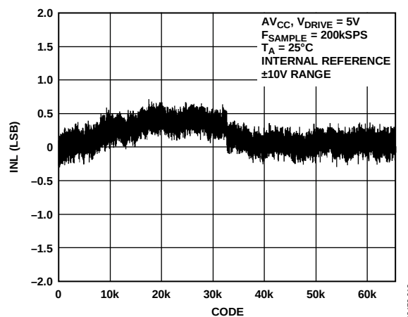
Figure 14. AD7606 Typical INL, \pm 10 V Range
