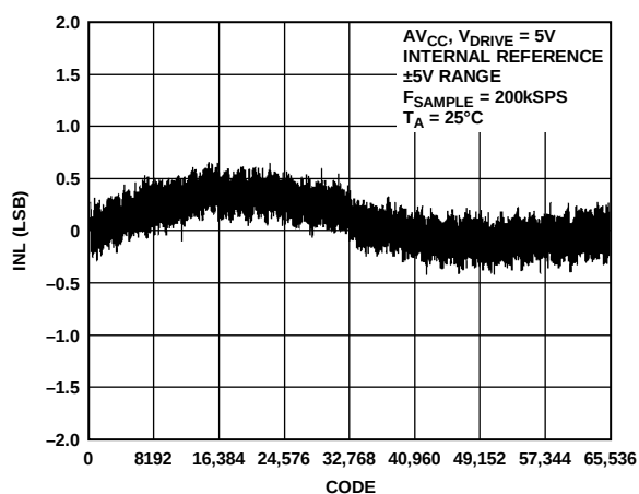
Figure 16. AD7606 Typical INL, \pm 5 V Range
