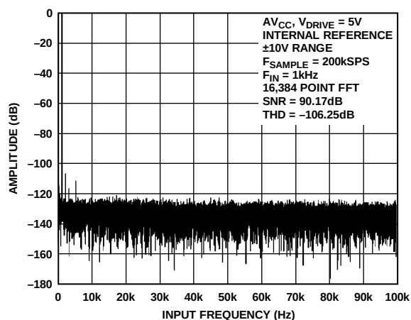
Figure 11. AD7606 FFT, \pm 10 V Range
