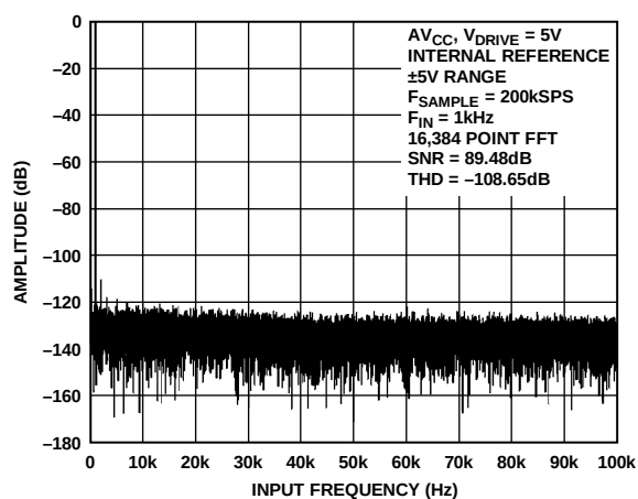
Figure 12. AD7606 FFT Plot, \pm 5 V Range
