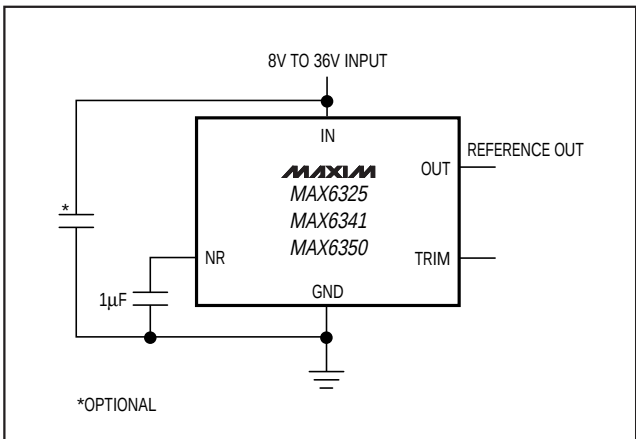
Figure 2. Noise-Reduction Capacitor
