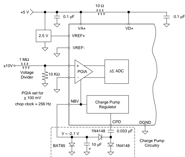
Figure 7. Input Ranges Greater than 5 V
