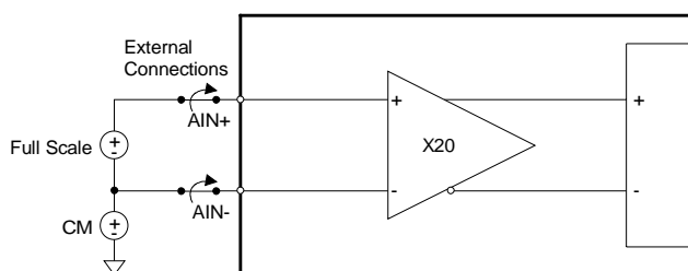
Figure 16. System Calibration of Gain (Low Ranges)
