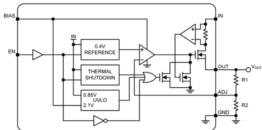
MIC47050 Adjustable Output Block Diagram
