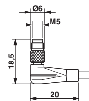
Plug M5 x 0.5, angled
