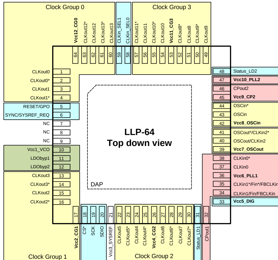
NKD Package 64-Pin WQFN Top View
