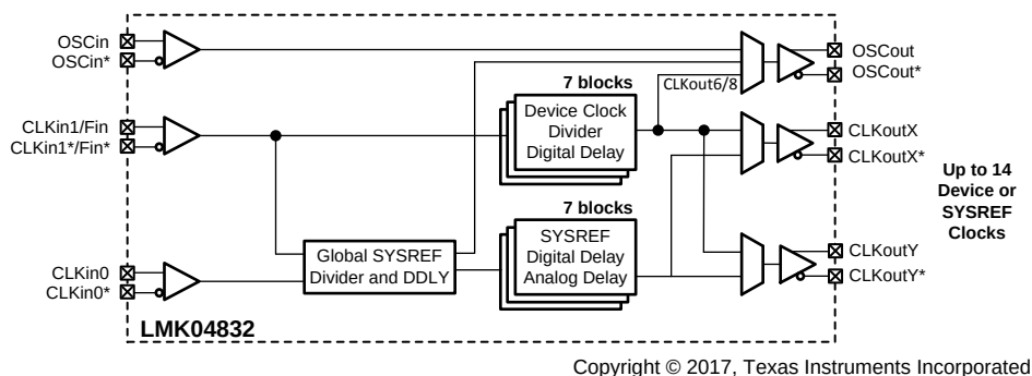
Figure 20. Simplified Functional Block Diagram for Distribution Mode
