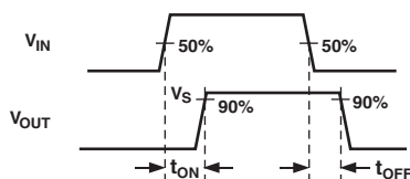
Test Circuit 4. Switching Times
