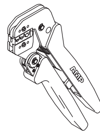
PRO-CRIMPER III Hand Crimping Tool (408-9252)
