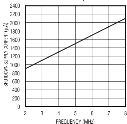
SHUTDOWN SUPPLY CURRENT vs. OSC FREQUENCY
