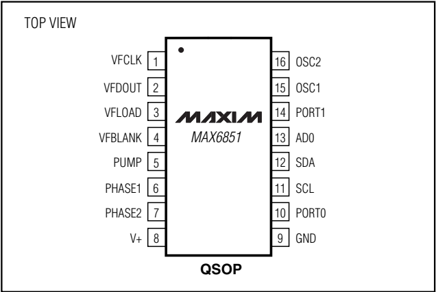
Pin Configuration
