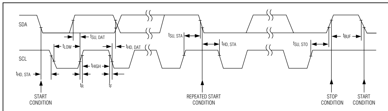
Figure 8. 2-Wire Serial Interface Timing Details
