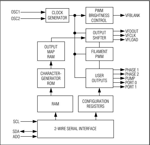
Functional Diagram
