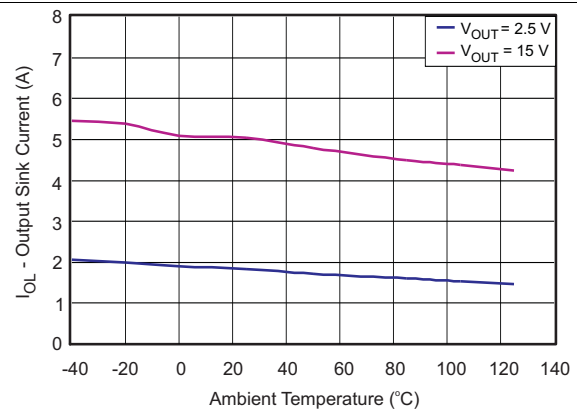
Figure 8. Output Sink Current vs. Temperature
