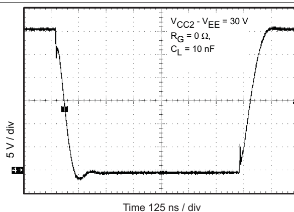
Figure 26. Output Waveform
