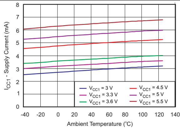
Figure 1. V_{CC1} Supply Current vs. Temperature
