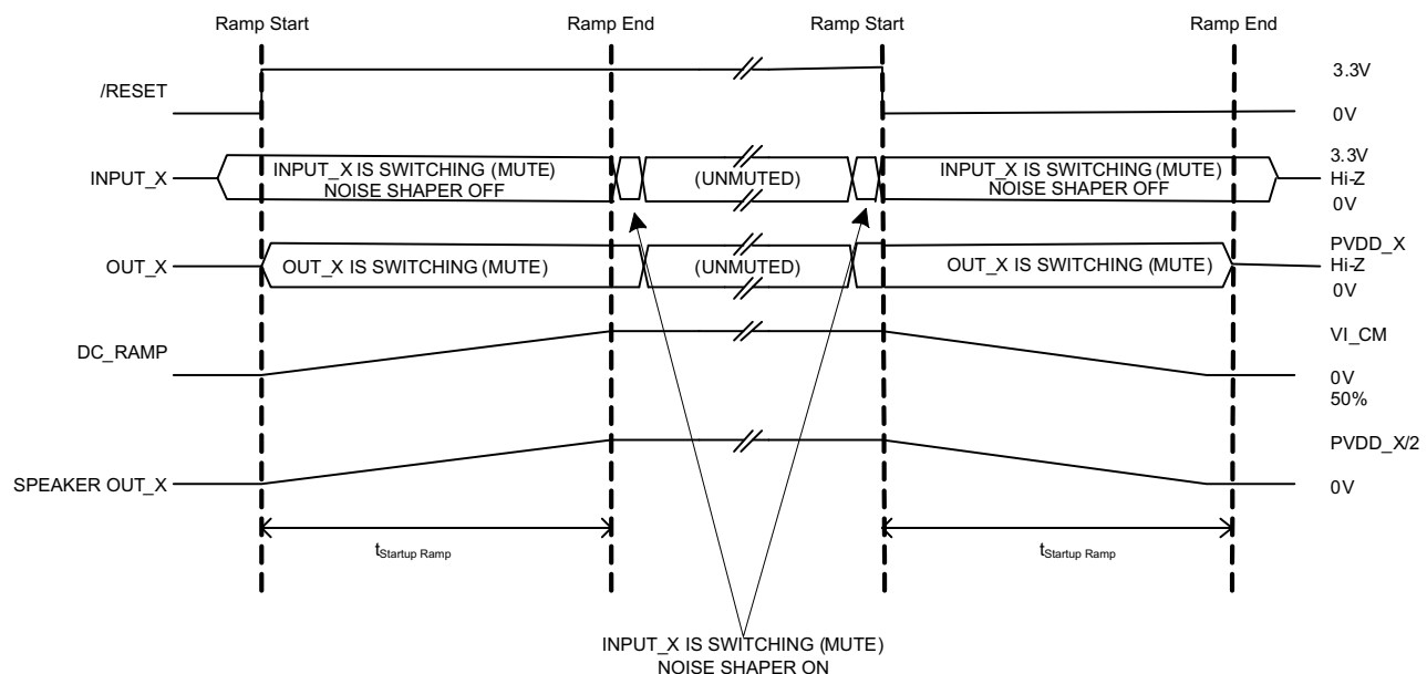
Figure 15. Start-up/Shutdown Ramp
