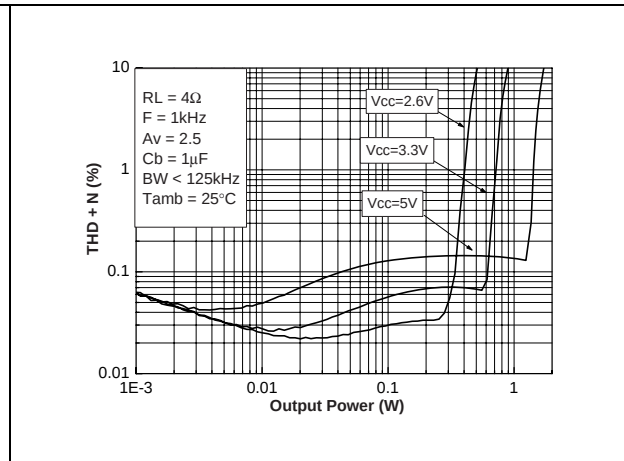
Figure 51. THD+N vs. output power
