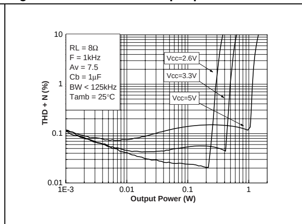
Figure 55. THD+N vs. output power
