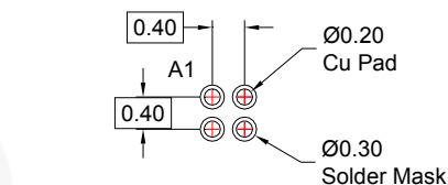
RECOMMENDED LAND PATTERN (NSMD PAD TYPE)
