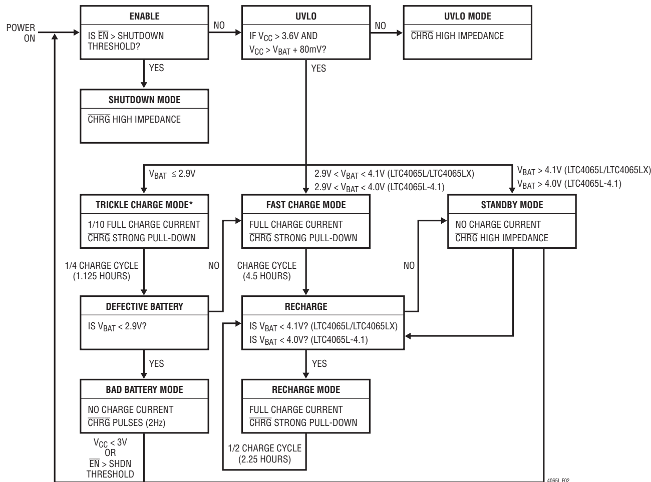
Figure 2. State Diagram of LTC4065L Operation
