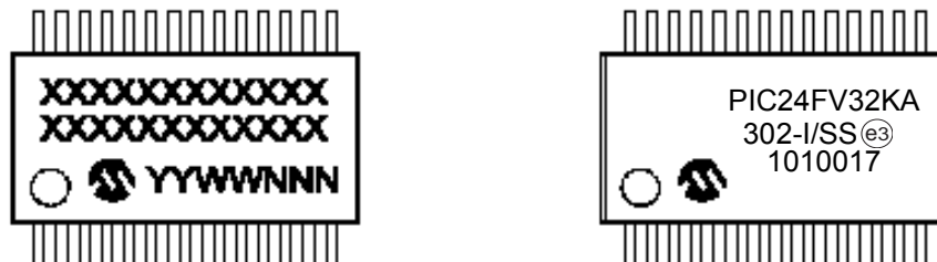
28-Lead SSOP (5.30 mm)
