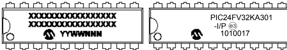
20-Lead PDIP (300 mil)
