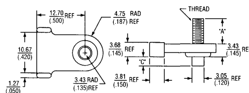
▲ FIGURE 5 TO-220 MOUNTS: 8190 SERIES
