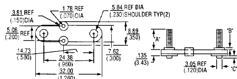
▲ FIGURE 1 TO-66 MOUNTS: 8160 SERIES
