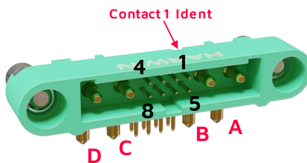
Male PCB mounted
