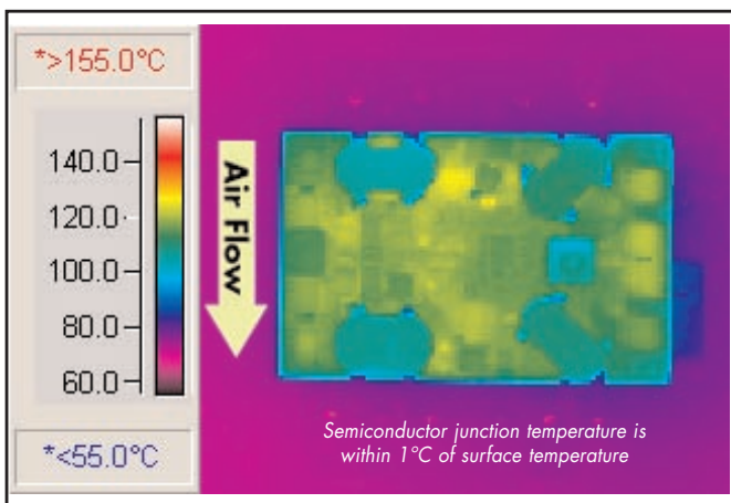
Figure 10: Thermal plot of converter at 15A load on 1.8V output and 12.5A load on 3.3V output with 70°C air flowing at 200 LFM. Air flow across the converter is from pin 1 to pin 3 (nominal input voltage).
