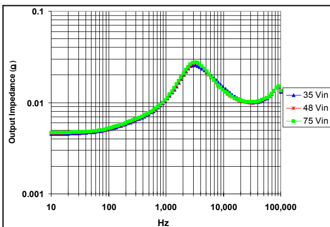
Figure 26: Output impedance ( Z_{out2} = V_{out2}/I_{out2} ) for minimum, nominal, and maximum input voltage at full rated power, for 3.3V output.
