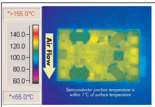
Figure 12: Thermal plot of converter at 13A load on 1.8V output and 10A load on 3.3V output with 85°C air flowing at 200 LFM. Air flow across the converter is from pin 1 to pin 3 (nominal input voltage).
