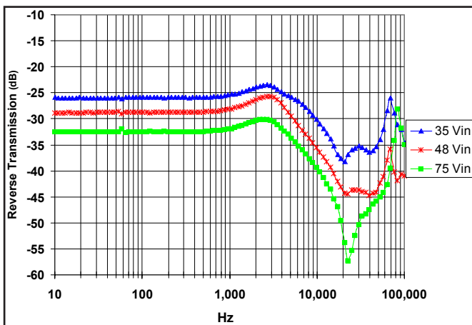
Figure 30: Reverse Transmission ( RT_2 = I_{in}/I_{out2} ) for minimum, nominal, and maximum input voltage at full rated power, for 3.3V output.
