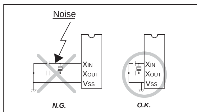
Fig. 89 Wiring for clock I/O pins
