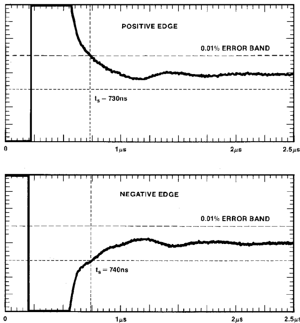
FIGURE 5: OP-42 Settling-Characteristics
