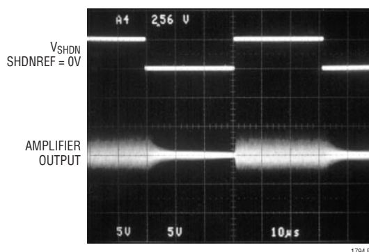
Figure 5. Shutdown and Recovery Timing
