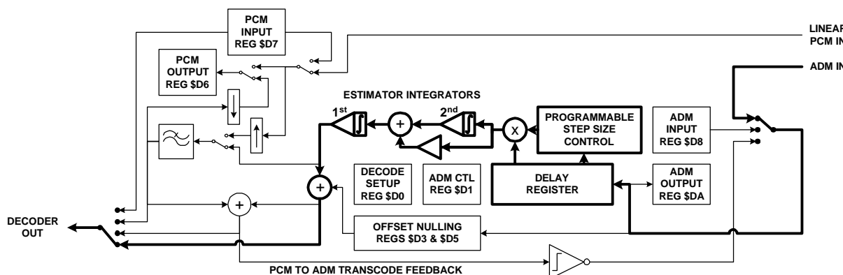
Figure 4 ADM Decoding
