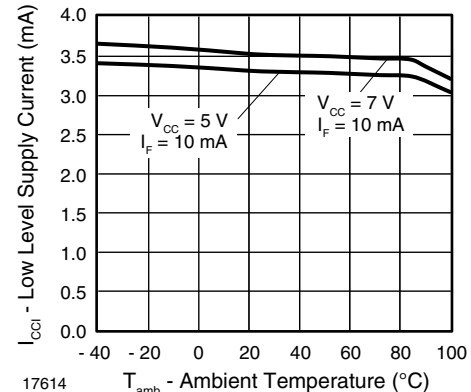
Fig. 9 - Low Level Supply Current vs. Ambient Temperature
