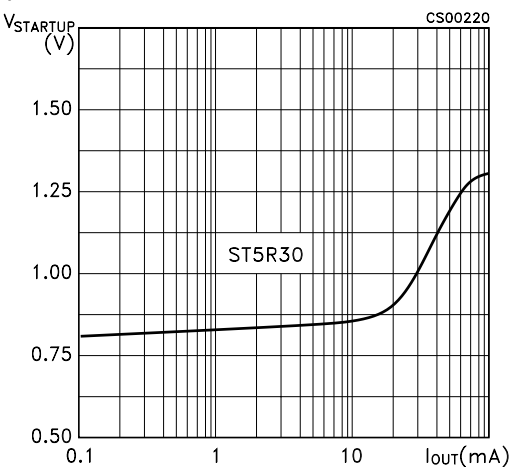
Figure 23: Start-up Voltage ( V_{IN} - V_F ) vs Output Current
