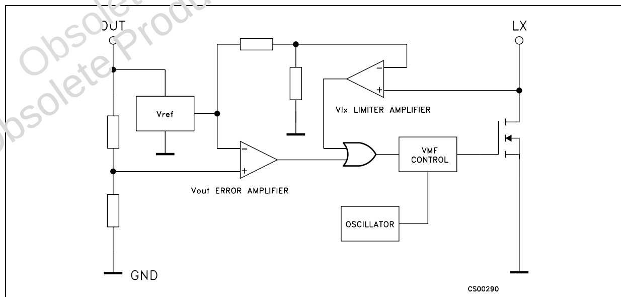
Figure 1: Schematic Diagram
