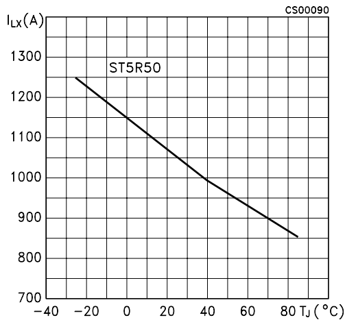
Figure 18: LX Switching Current Limit vs Temperature
