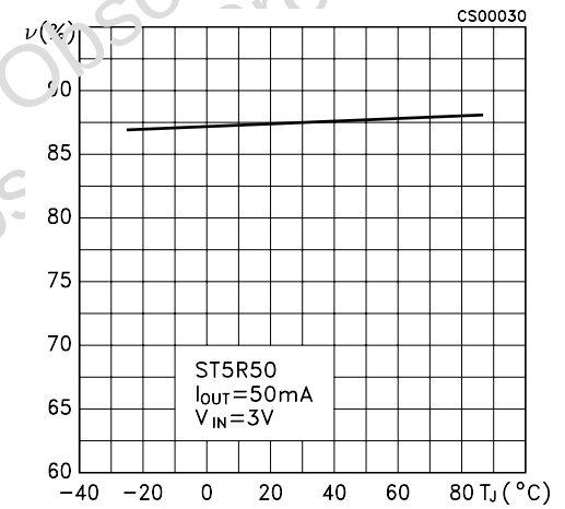
Figure 11: Efficiency vs Temperature
