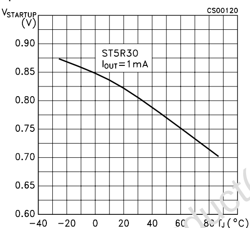
Figure 21: Start-up Voltage ( V_{IN} - V_F ) vs Temperature
