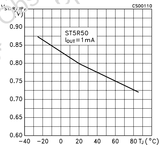
Figure 20: Start-up Voltage ( V_{IN} - V_F ) vs Temperature
