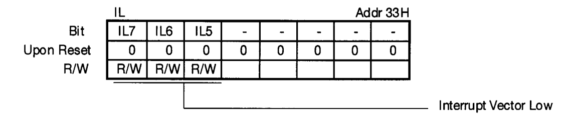
Figure 57. Interrupt Vector Low Register
