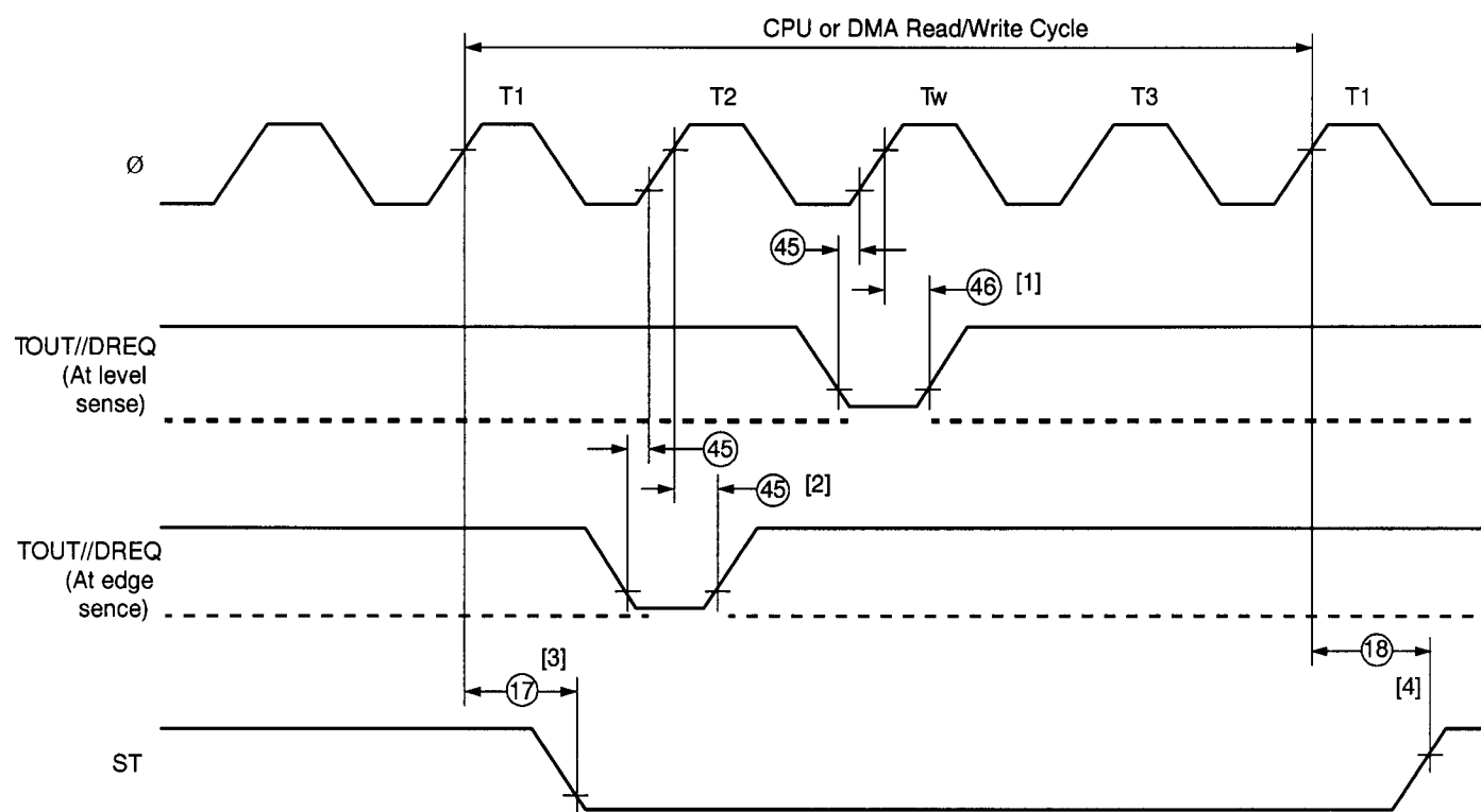
Figure 6. CPU Timing
