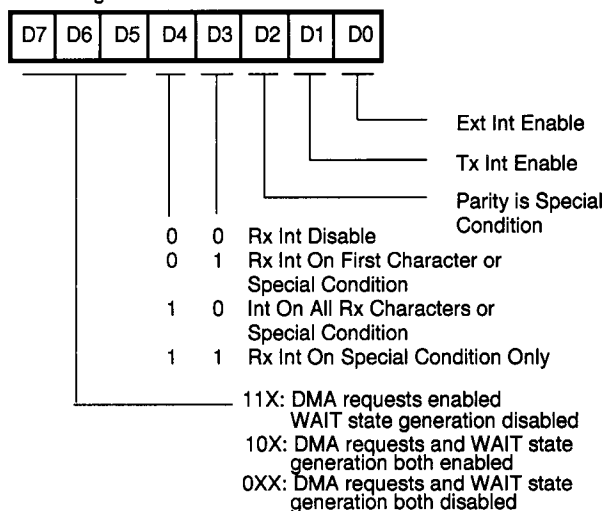
Figure 68. Write Register Bit Functions
