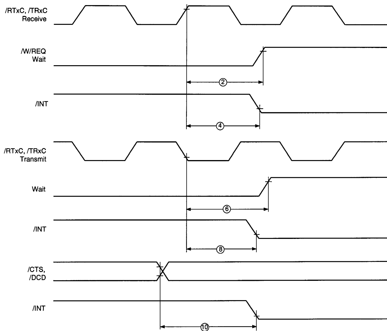
Figure 18. EMSCC System Timing
