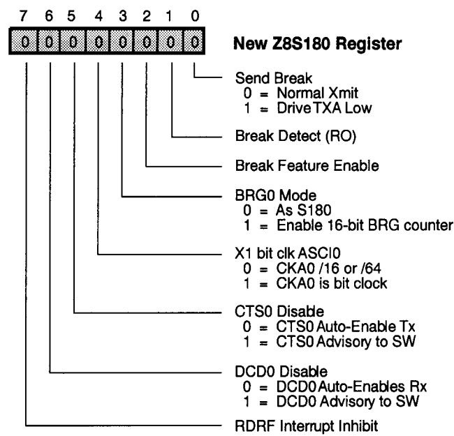
Figure 32. ASCII0 Extension Control Register (I/O Address 12)
