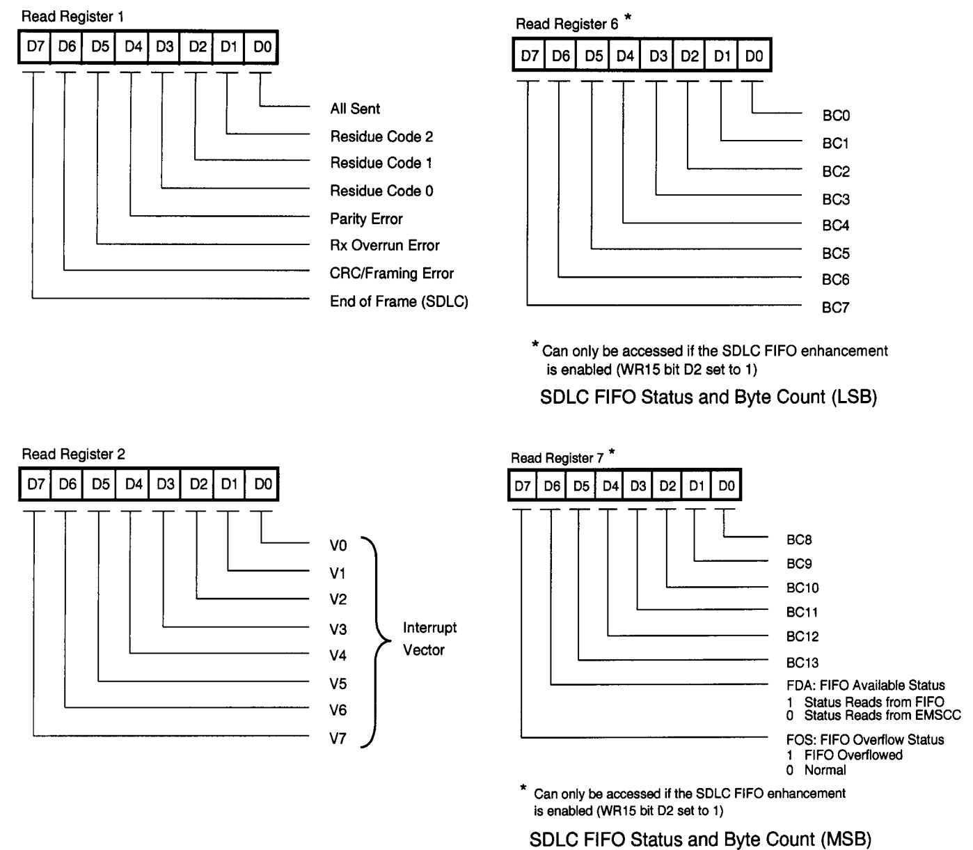
Figure 72. Read Register Bit Functions
