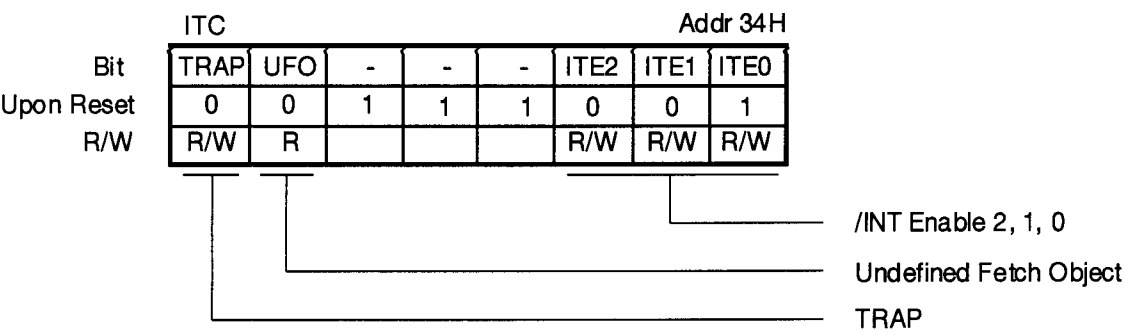
Figure 58. INT/TRAP Control Register
