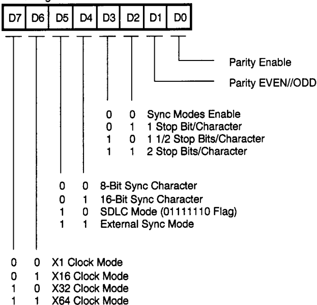
Figure 68. Write Register Bit Functions
