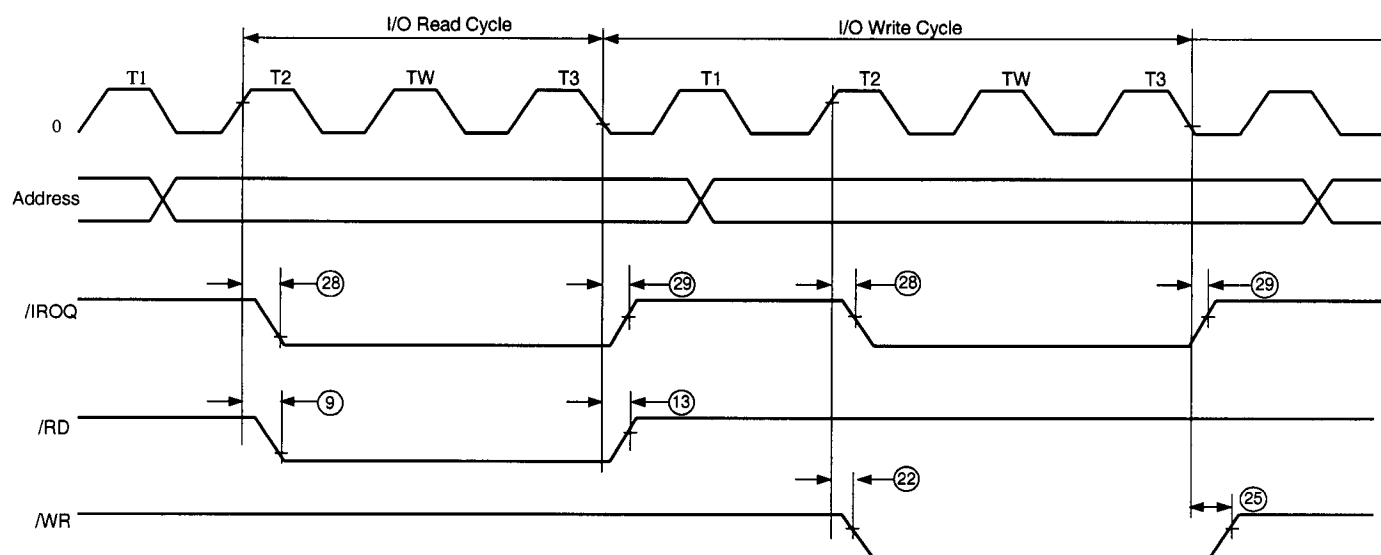
Figure 6. CPU Timing
