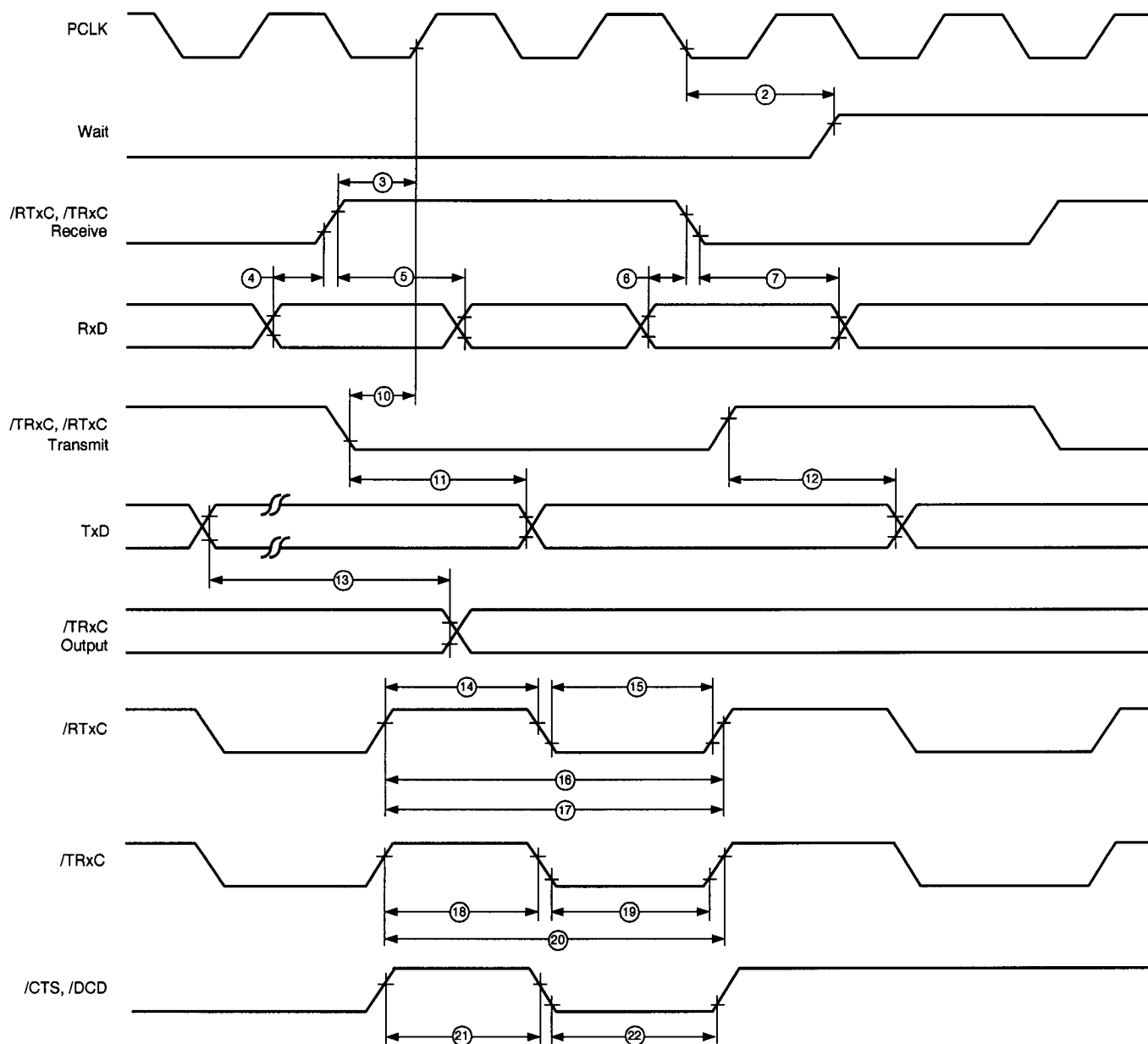
Figure 17. EMSCC General Timing Diagram
