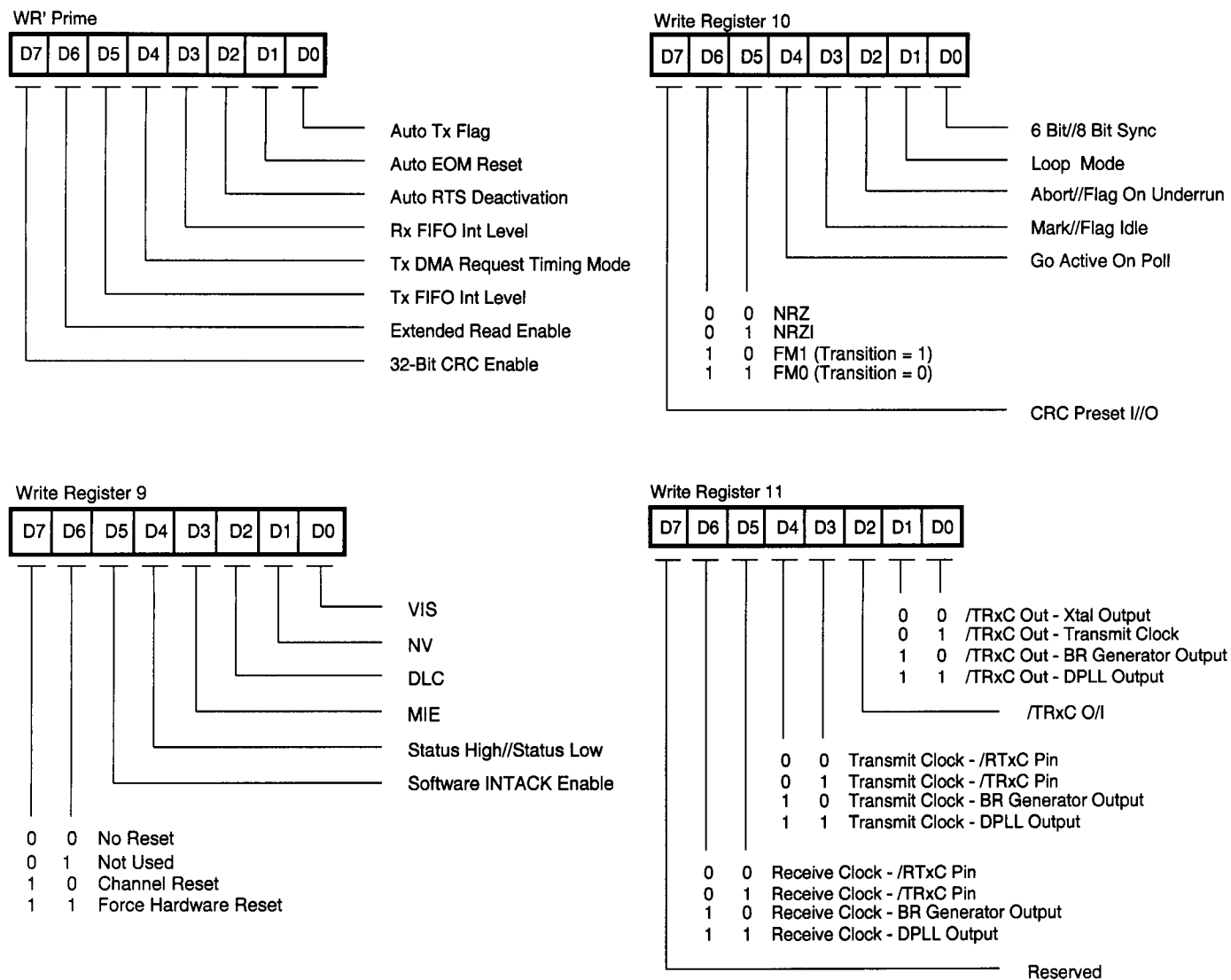
Figure 70. Write Register Bit Functions (Continued)
