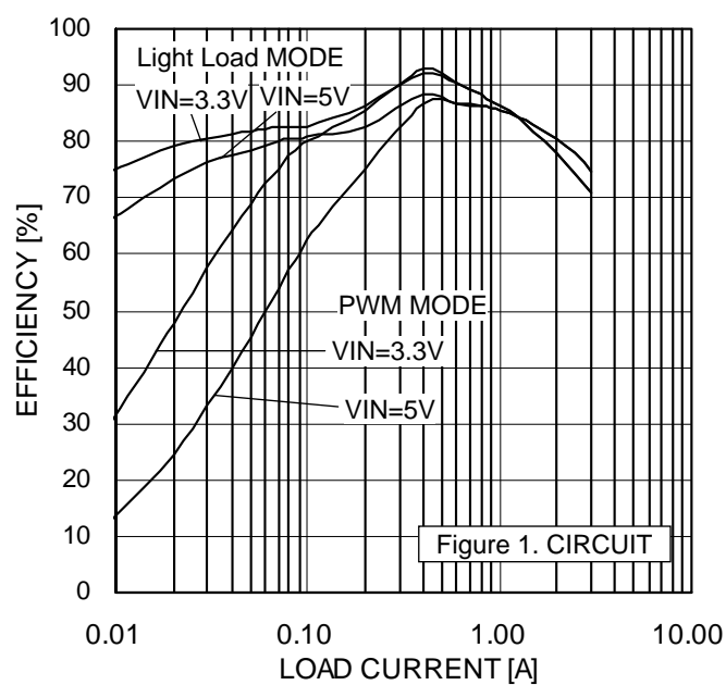
Figure 8. Efficiency(BD90525EFJ-C)
